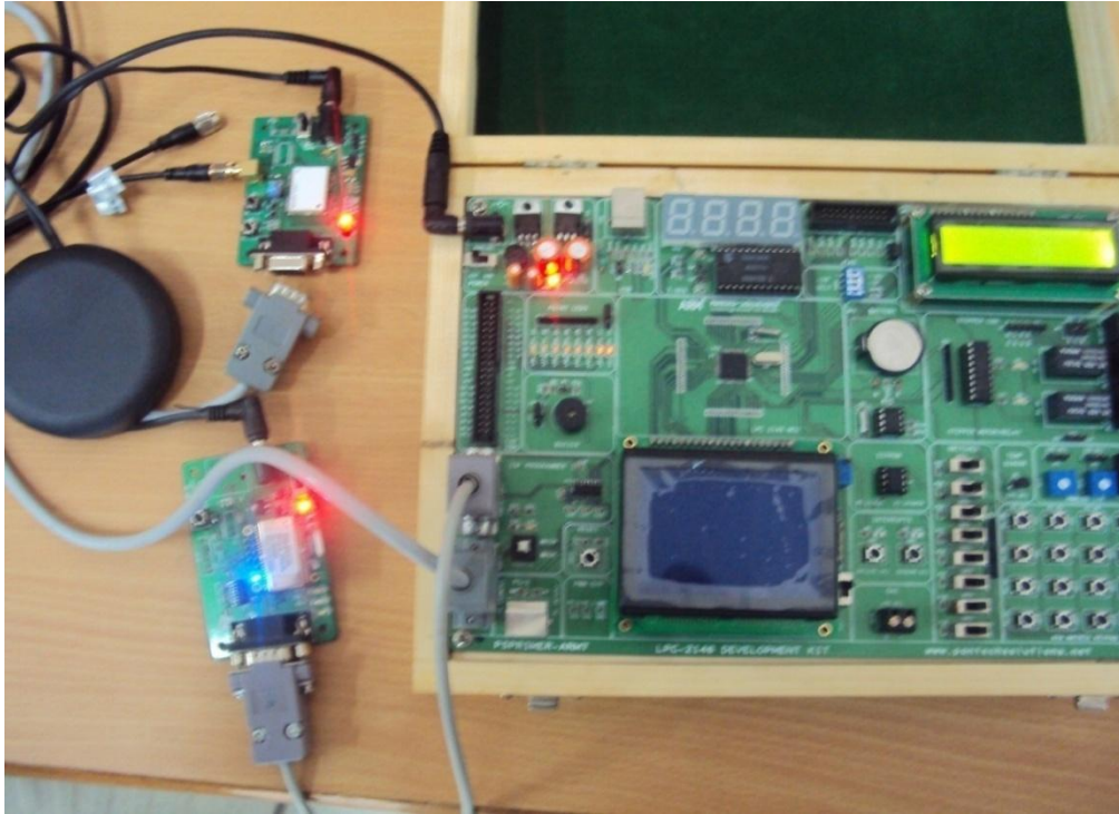
Experimental setup using ARM Development Board
